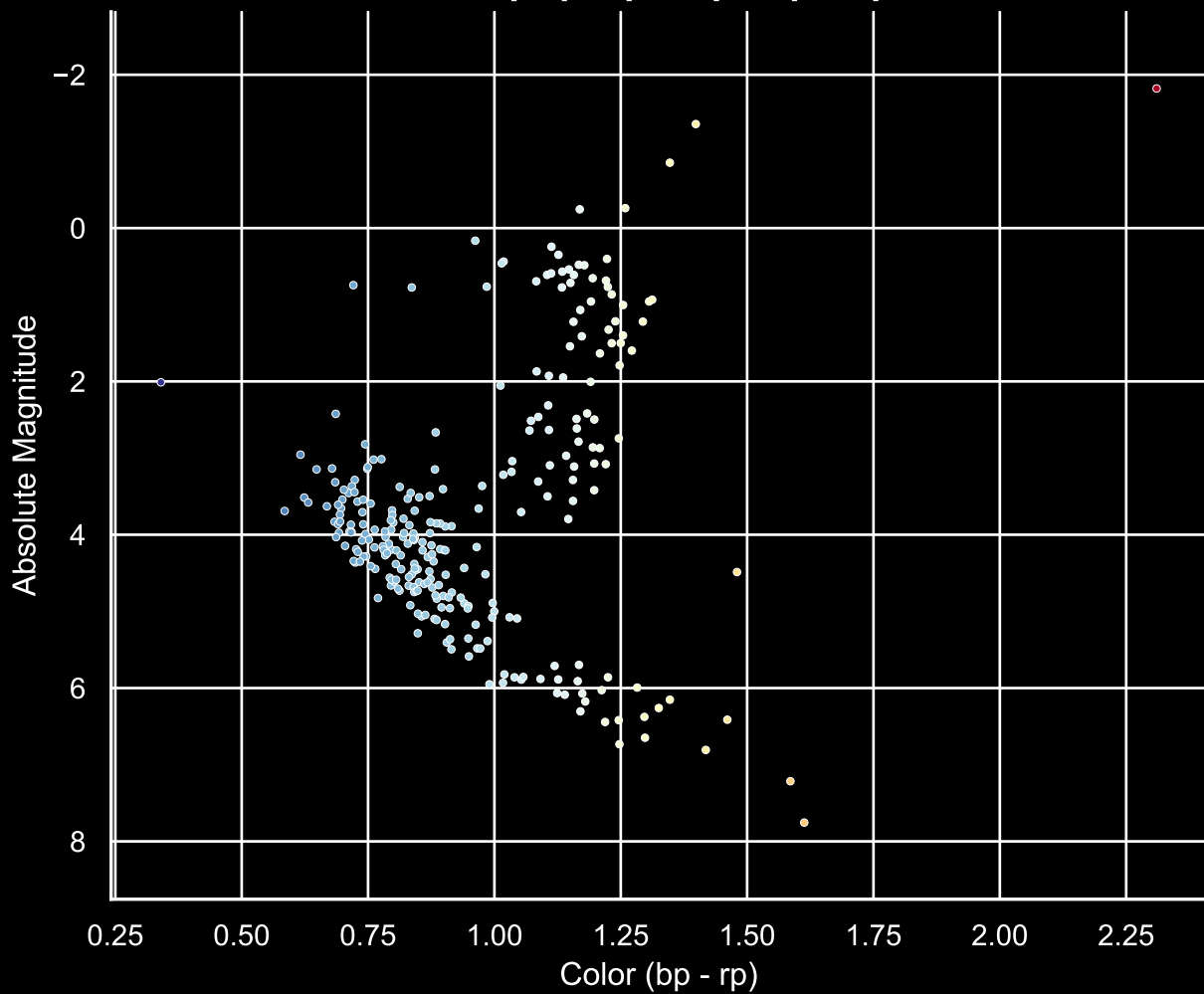
GALAH Hertzsprung-Russel Diagram Field [109] Ra [328.92] Dec [-66.38]
