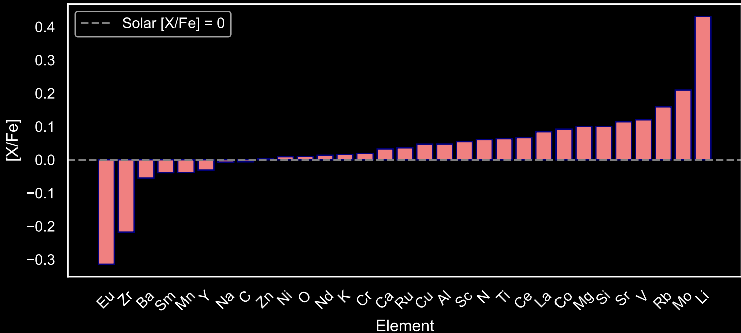
Abundance Pattern for GALAH Main Sequence Stars: Star Field [109] (N=132)
