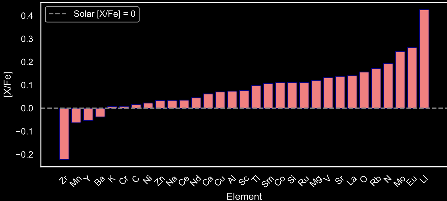
Abundance Pattern for GALAH Star Field [109] (N=279)
