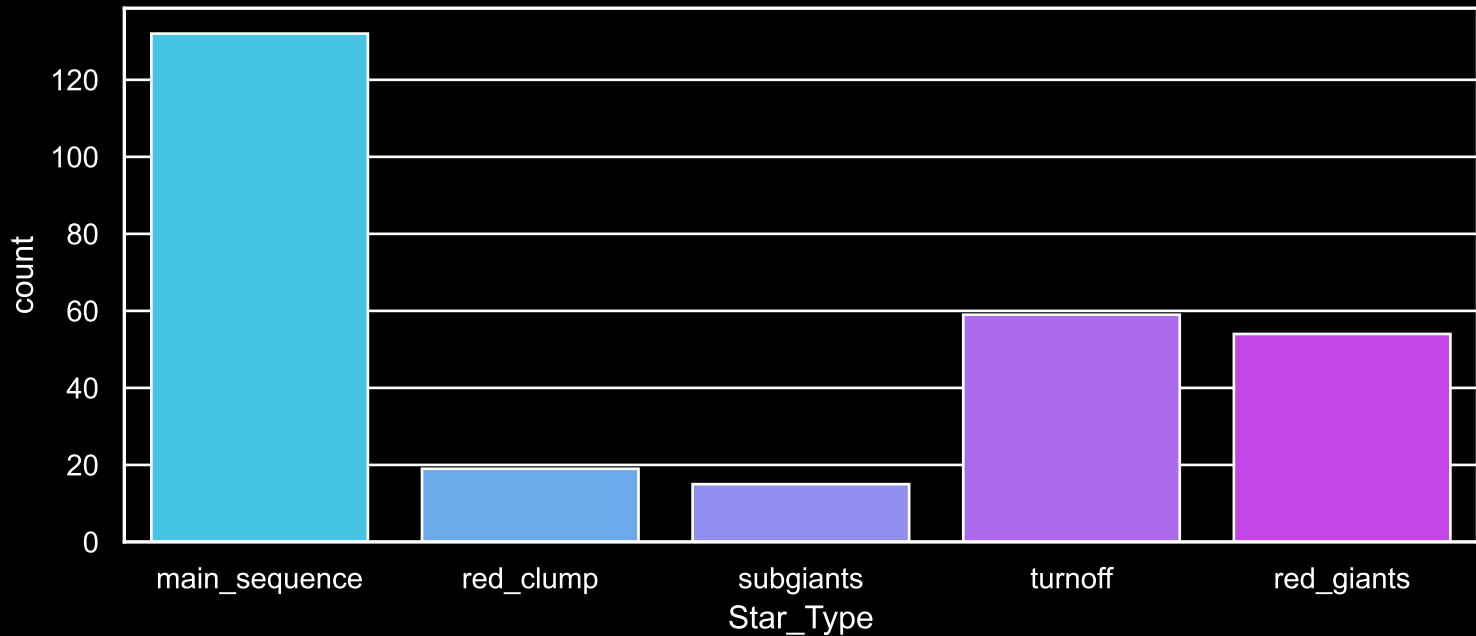
Field [109] Count plot of Star Type
