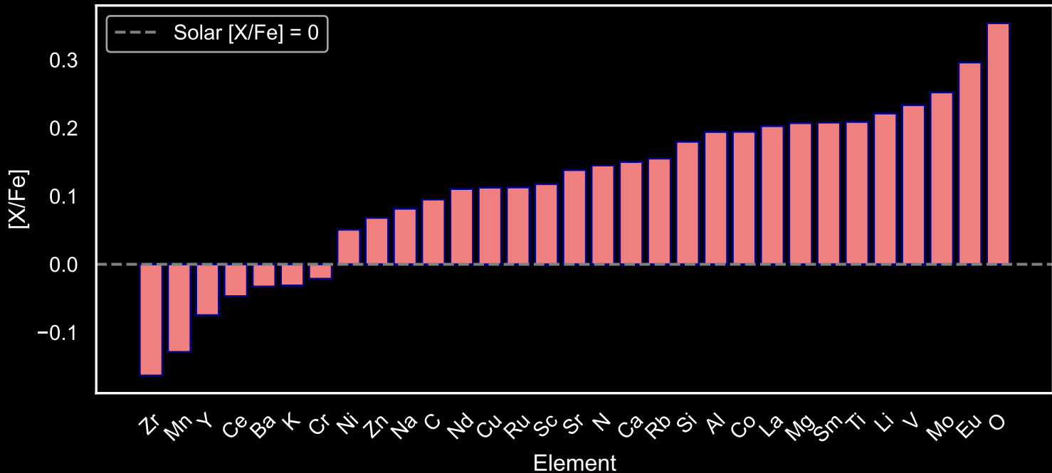
Abundance Pattern for GALAH Red Giants: Star Field [109] (N=73)
